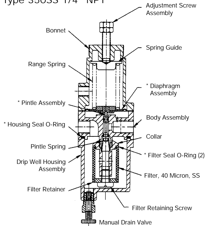
Type 350SS 1/4" NPT
