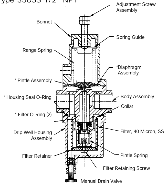
Type 350SS 1/2" NPT
