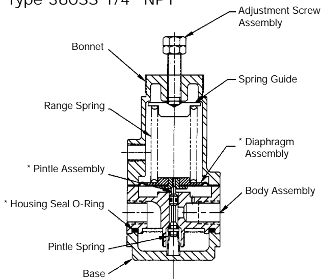
Type 360SS 1/4" NPT
